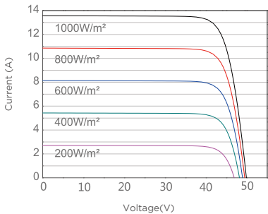
Current-Voltage Curve(UE540M-72H)
