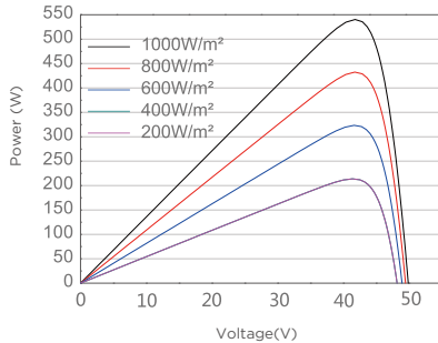
Current-Voltage Curve(UE540M-72H)
